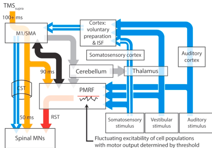
Fig. 4. | A hypothesized model for the brain circuits subserving the expression of long latency stretch reflexes. Transcortical contributions to long latency stretch reflexes are enabled by a pathway that incorporates the primary somatosensory and motor cortices before descending to muscles through the corticospinal tract (white arrows). Stimulation of somatosensory, vestibular, or auditory systems results in the transfer of these signals to the cortex and the pontomedullary reticular formation (blue arrows), each of which has thresholds for activating output cells. Inhibition of the primary motor cortex (or areas involved in movement preparation) by application of suprathreshold TMS (orange arrows) results in almost synchronous inhibition of cells within the spinal cord and PMRF, although for different times. Spinal motoneurons appear to be inhibited for ~50 ms after TMS. Output cells inside the motor cortex, however, can be blocked for up to 200 ms (Strick, 1983). During periods of cortical inhibition, activation of the corticospinal tract is not possible, although a combination of cortico-reticulospinal input (black arrows) and sufficiently large sensory input can still activate reticulospinal tract cells (red arrow) after any TMS-induced inhibition of PMRF ceases. The likelihood of PMRF output (startle) is controlled in this model by the magnitude of the sensory input and the immediate excitability of PMRF cells. A comparable situation is expected to arise at the cortical level (see Alibiglou and MacKinnon, 2012). Task, posture, and stability-dependent modulation of stretch reflex reactions likely entail input from the cerebellum to both the main motor cortex and reticular formation (gray arrows). In this figure, thalamocortical projections reach regions involved for voluntary motor preparation, although projections straight to M1 may also play an essential role in modulating quick responses. M1, Primary motor cortex; SMA, supplementary motor region; PMRF, pontomedullary reticular formation; ISF, intersensory facilitation; MN, motoneuron (adapted from Shemmell, J., 2015).
